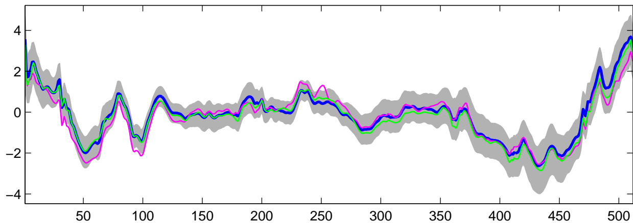
Estimated U_{17}(t) using G-WFMM: DE data, run 5
