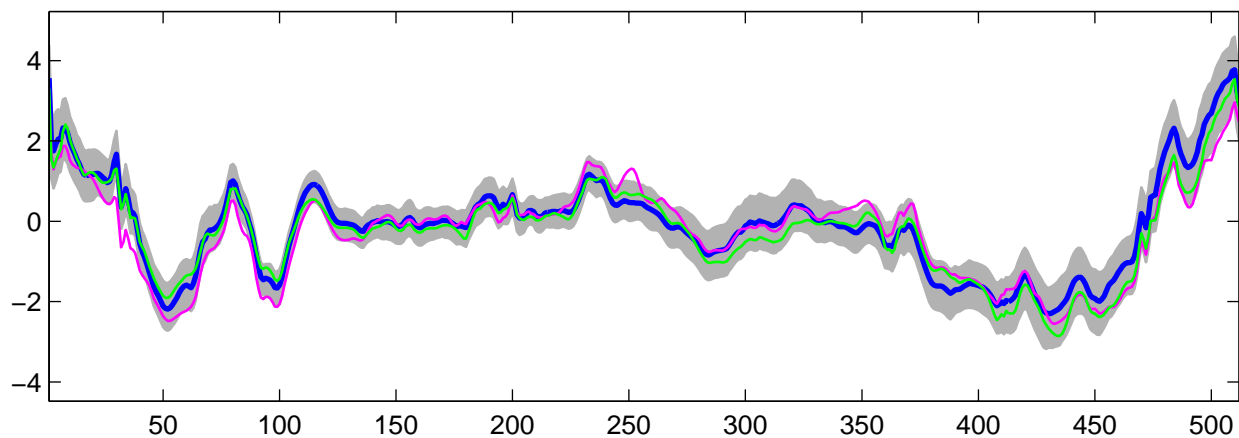
Estimated U_{17}(t) using R-WFMM: DE data, run 5
