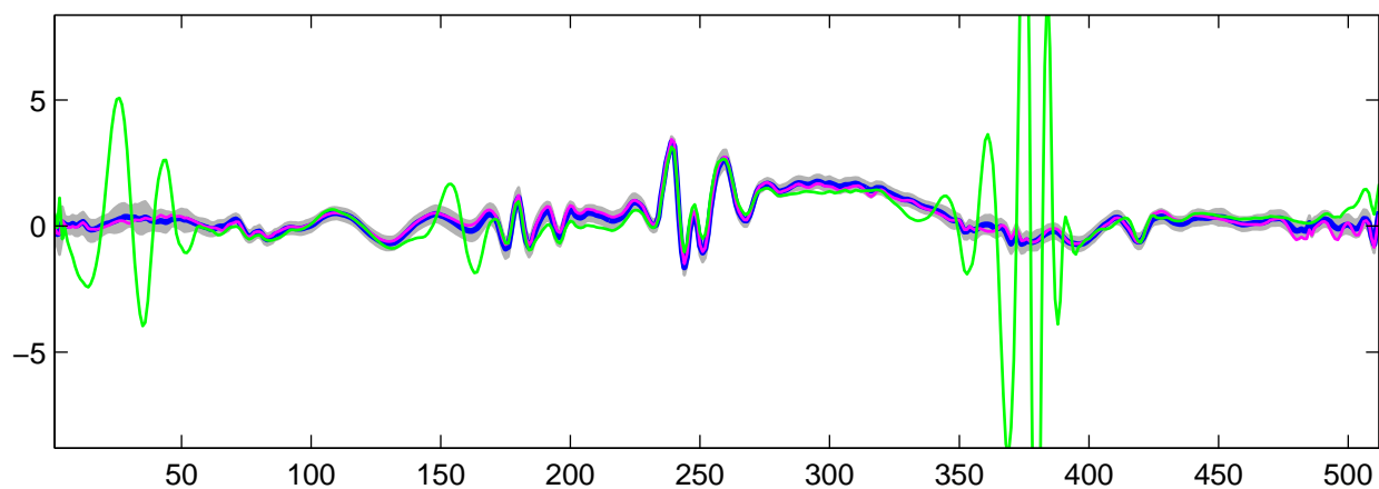
Estimated U_{17}(t) using R-WFMM: t_1 data, run 5
