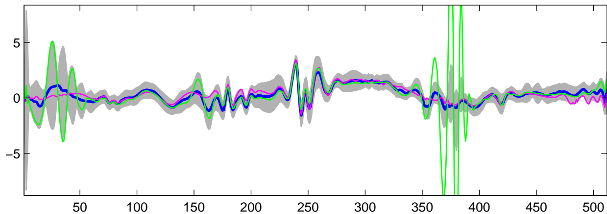
Estimated U_{17}(t) using G-WFMM: t_1 data, run 5
