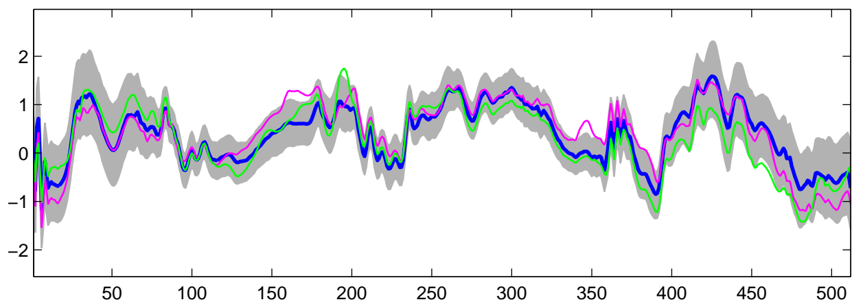
Estimated U_{17}(t) using R-WFMM: t_3 data, run 5
