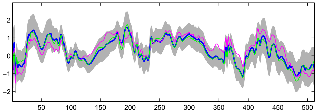
Estimated U_{17}(t) using G-WFMM: t_3 data, run 5
