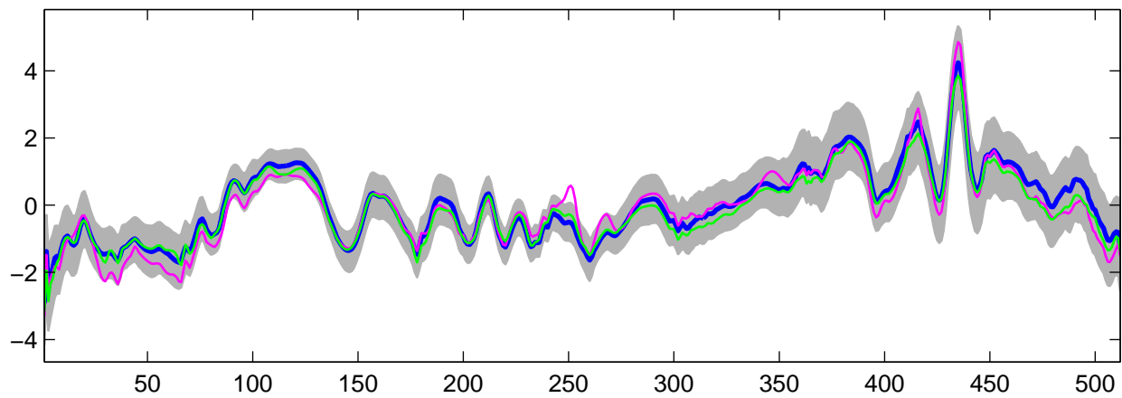
Estimated U_{18}(t) using G-WFMM: DE data, run 5
