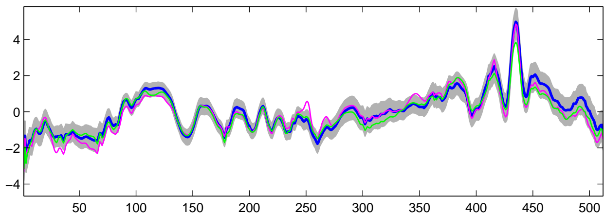
Estimated U_{18}(t) using R-WFMM: DE data, run 5
