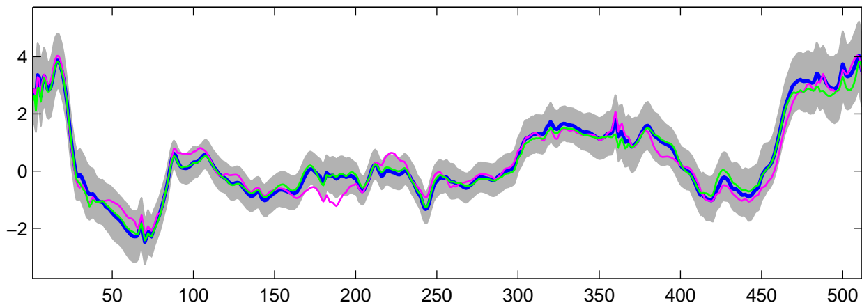
Estimated U_{18}(t) using G-WFMM: Normal data, run 5
