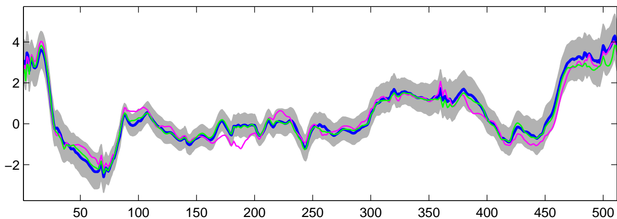
Estimated U_{18}(t) using R-WFMM: Normal data, run 5
