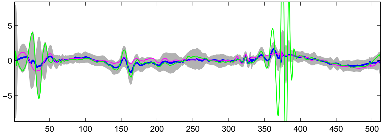
Estimated U_{18}(t) using G-WFMM: t_1 data, run 5
