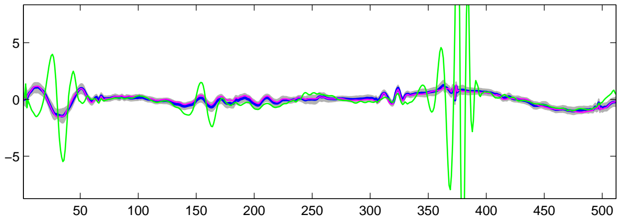
Estimated U_{18}(t) using R-WFMM: t_1 data, run 5
