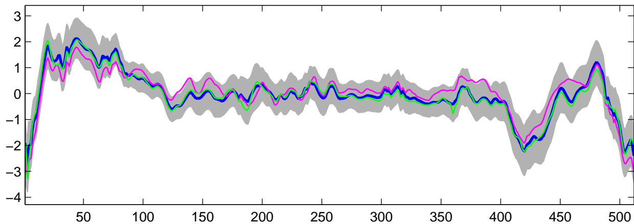
Estimated U_{18}(t) using G-WFMM: t_3 data, run 5
