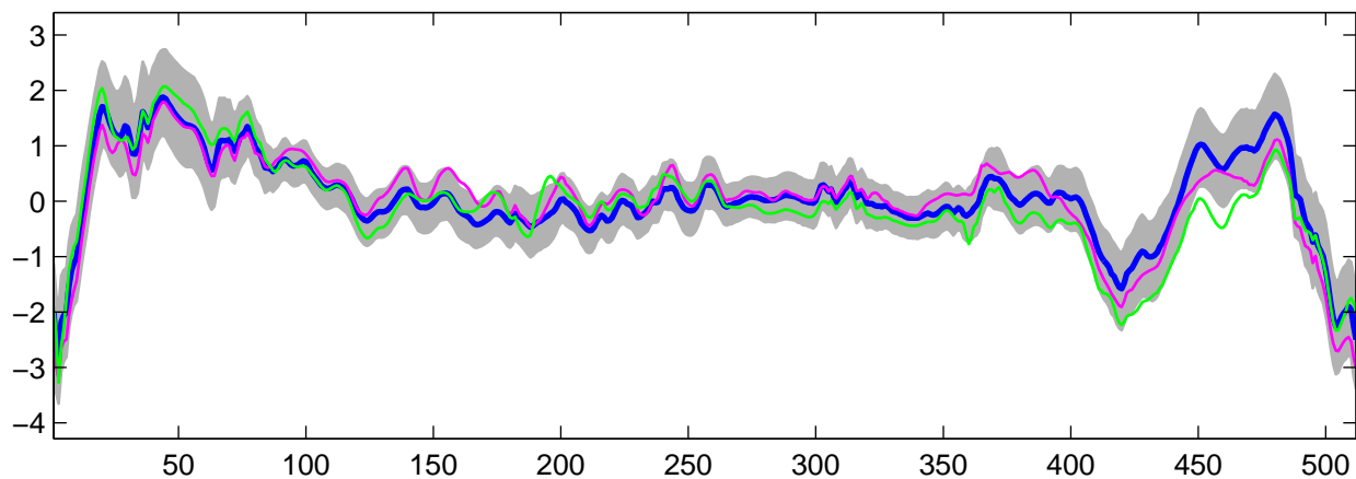
Estimated U_{18}(t) using R-WFMM: t_3 data, run 5
