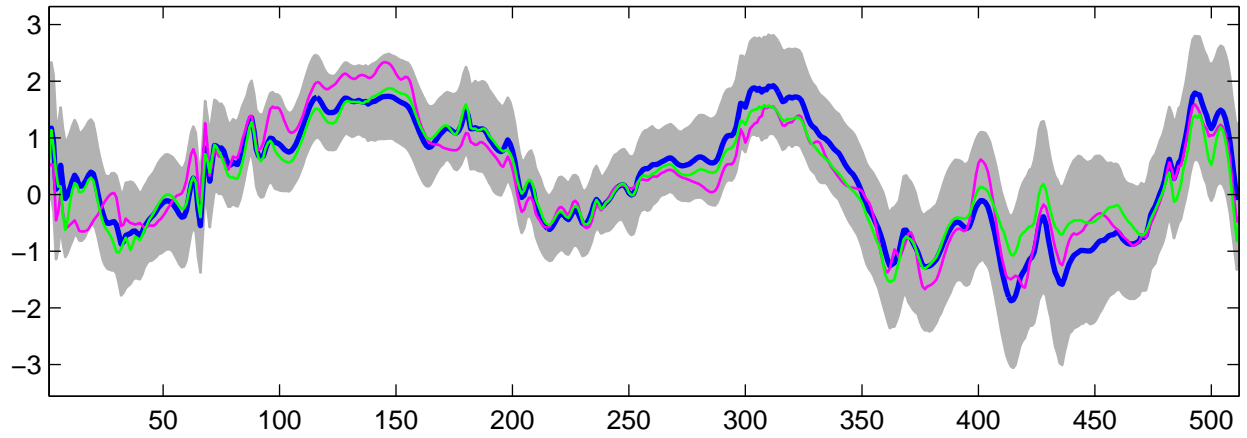
Estimated U_{19}(t) using G-WFMM: DE data, run 5
