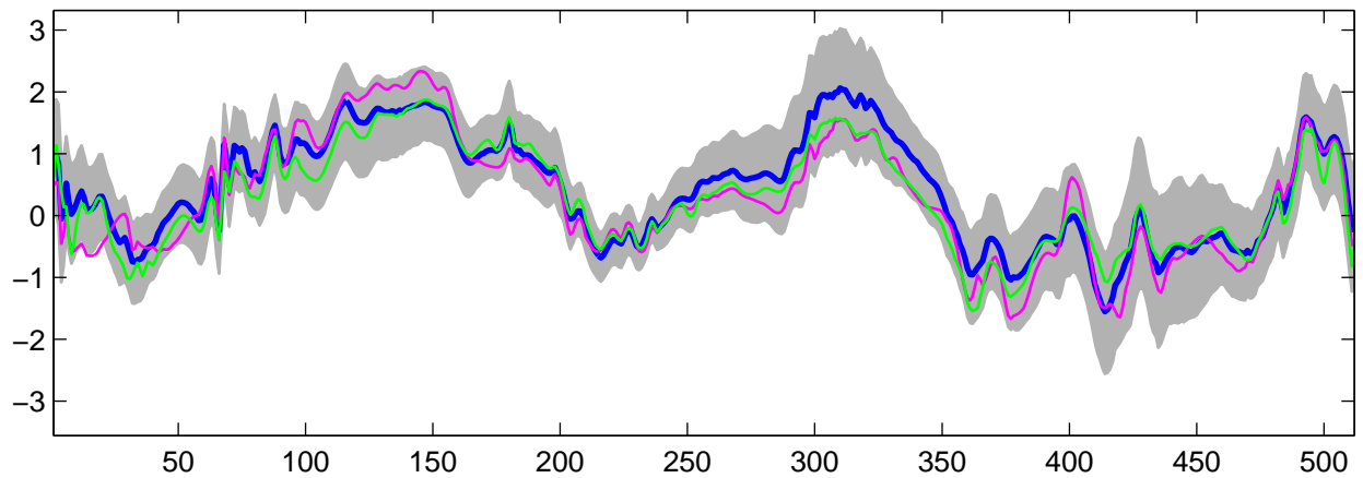
Estimated U_{19}(t) using R-WFMM: DE data, run 5
