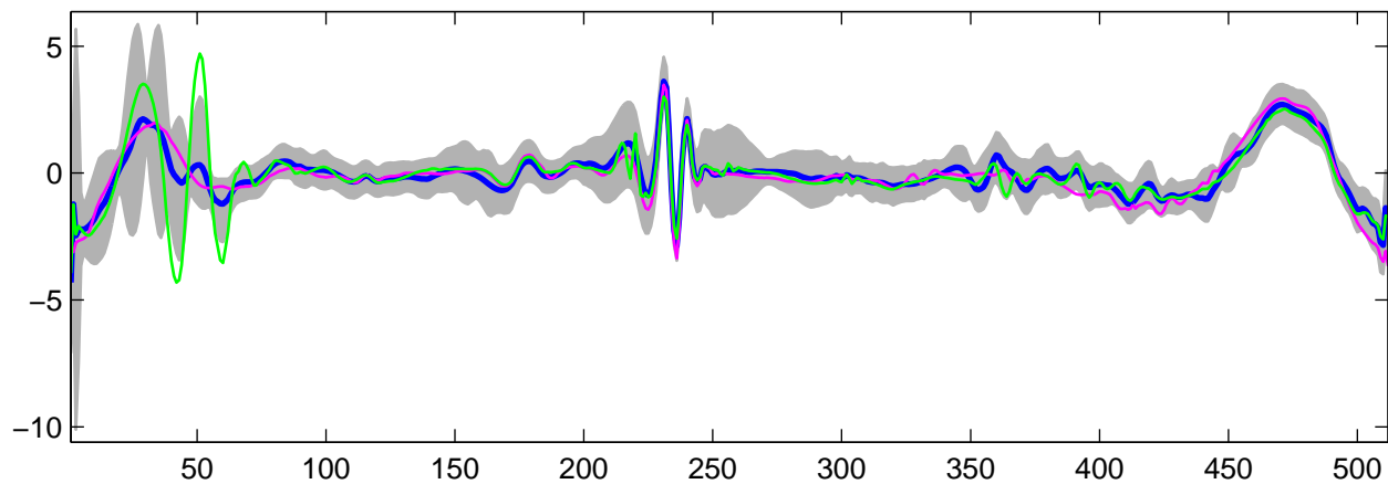
Estimated U_{19}(t) using G-WFMM: t_1 data, run 5
