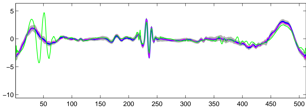
Estimated U_{19}(t) using R-WFMM: t_1 data, run 5
