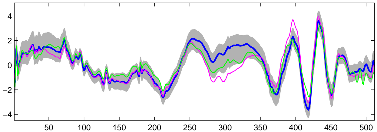
Estimated U_{19}(t) using R-WFMM: t_2 data, run 5
