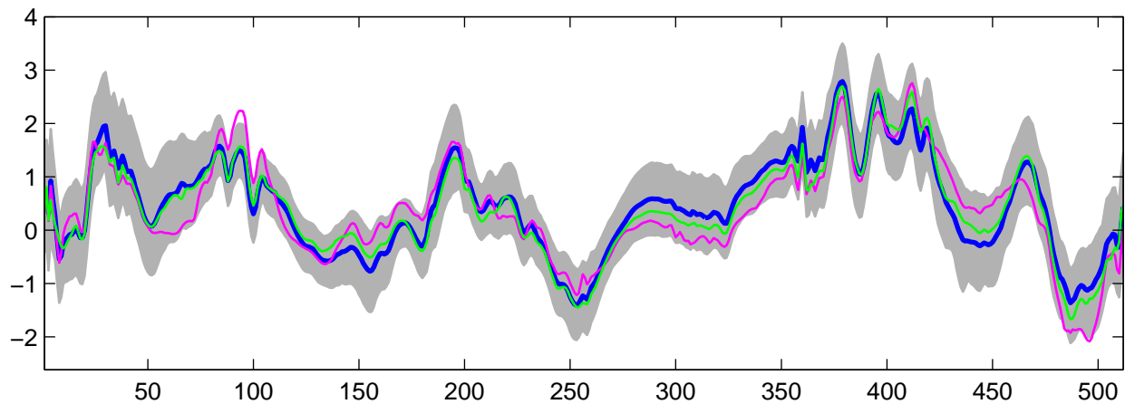
Estimated U_{19}(t) using G-WFMM: t_3 data, run 5
