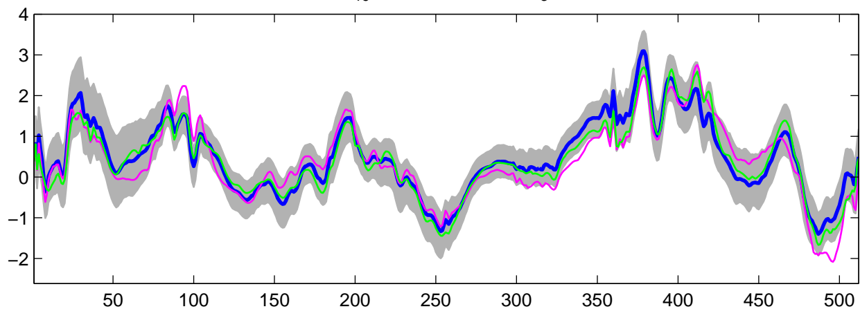
Estimated U_{19}(t) using R-WFMM: t_3 data, run 5
