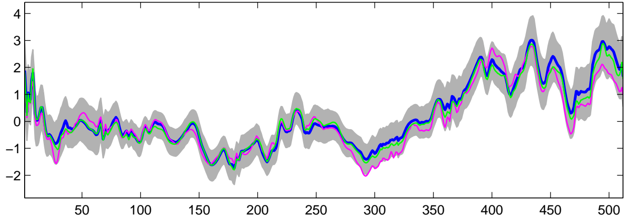
Estimated U_1(t) using G-WFMM: Normal data, run 5
