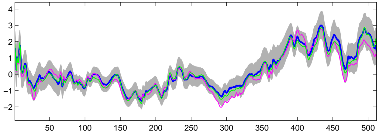
Estimated U_1(t) using R-WFMM: Normal data, run 5
