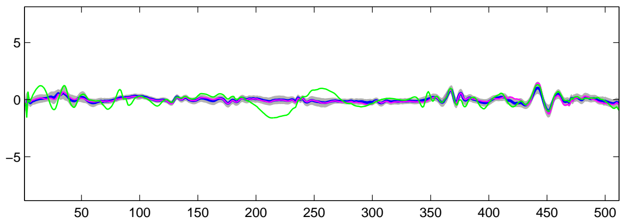
Estimated U_1(t) using R-WFMM: t_1 data, run 5
