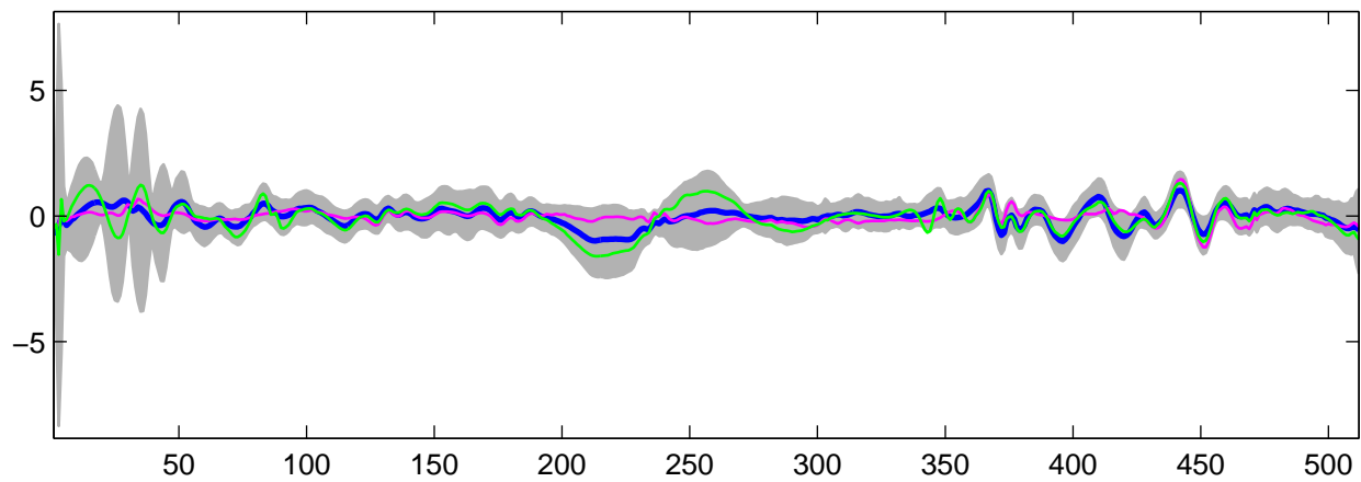
Estimated U_1(t) using G-WFMM: t_1 data, run 5
