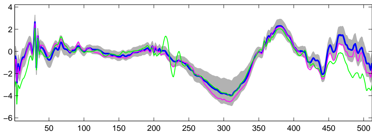
Estimated U_1(t) using R-WFMM: t_2 data, run 5
