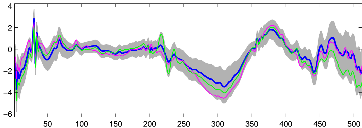
Estimated U_1(t) using G-WFMM: t_2 data, run 5
