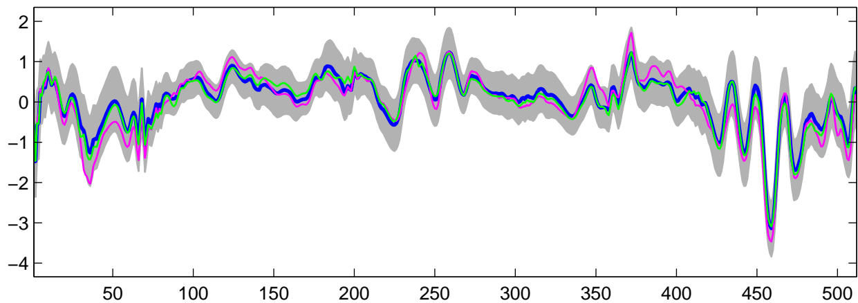
Estimated U_1(t) using G-WFMM: t_3 data, run 5
