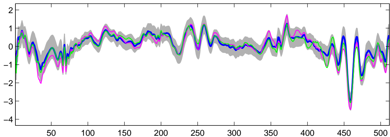
Estimated U_1(t) using R-WFMM: t_3 data, run 5
