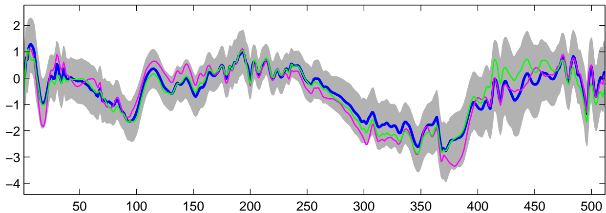
Estimated U_{20}(t) using G-WFMM: DE data, run 5
