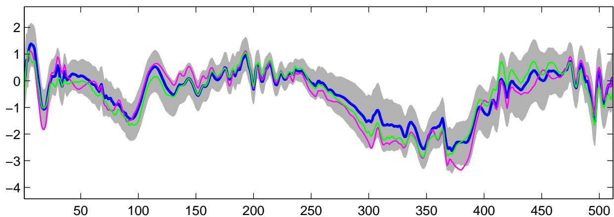
Estimated U_{20}(t) using R-WFMM: DE data, run 5
