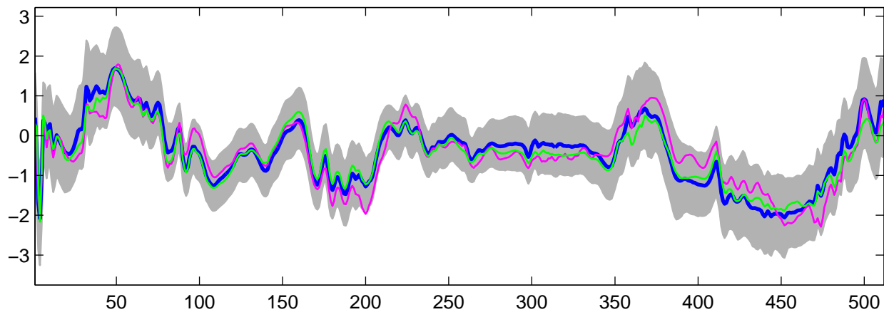
Estimated U_{20}(t) using G-WFMM: Normal data, run 5
