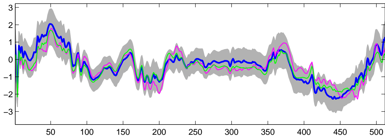
Estimated U_{20}(t) using R-WFMM: Normal data, run 5
