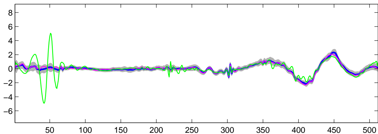
Estimated U_{20}(t) using R-WFMM: t_1 data, run 5
