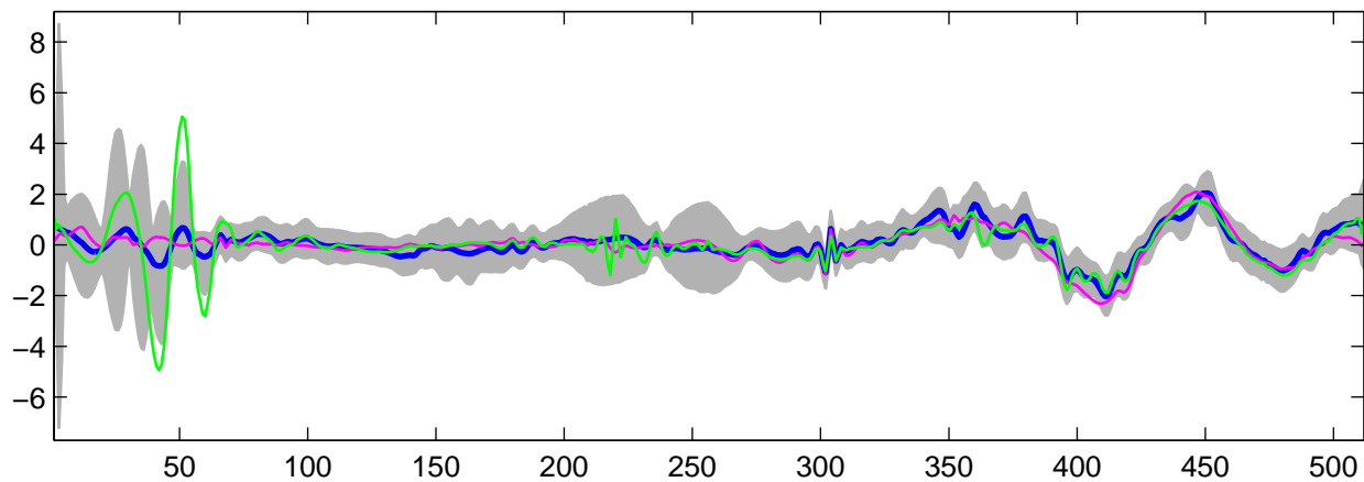
Estimated U_{20}(t) using G-WFMM: t_1 data, run 5
