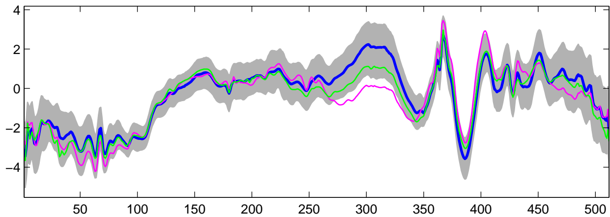
Estimated U_{20}(t) using G-WFMM: t_2 data, run 5
