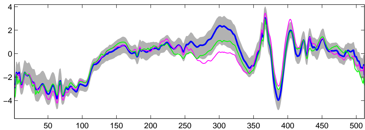
Estimated U_{20}(t) using R-WFMM: t_2 data, run 5
