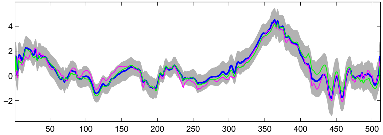
Estimated U_{21}(t) using G-WFMM: DE data, run 5
