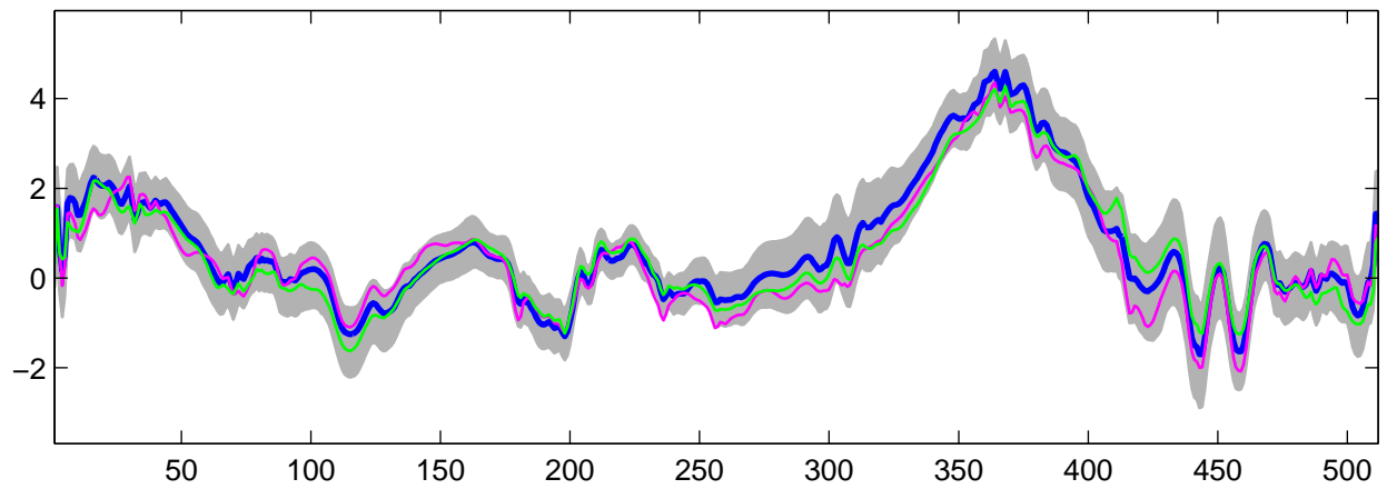
Estimated U_{21}(t) using R-WFMM: DE data, run 5
