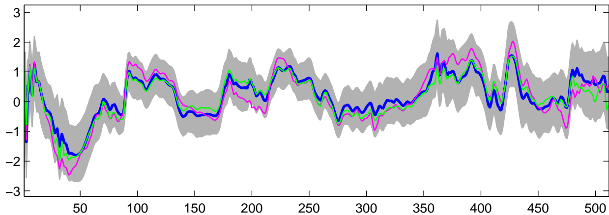
Estimated U_{21}(t) using G-WFMM: Normal data, run 5
