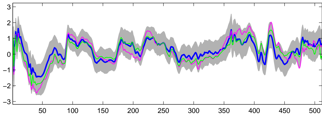
Estimated U_{21}(t) using R-WFMM: Normal data, run 5
