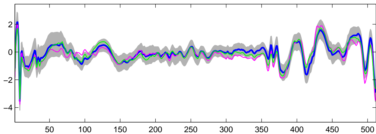
Estimated U_{21}(t) using R-WFMM: t_3 data, run 5
