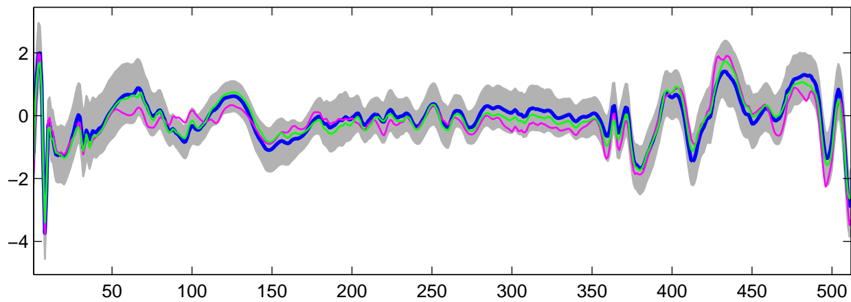
Estimated U_{21}(t) using G-WFMM: t_3 data, run 5
