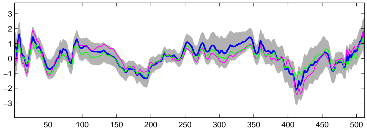
Estimated U_{22}(t) using R-WFMM: DE data, run 5
