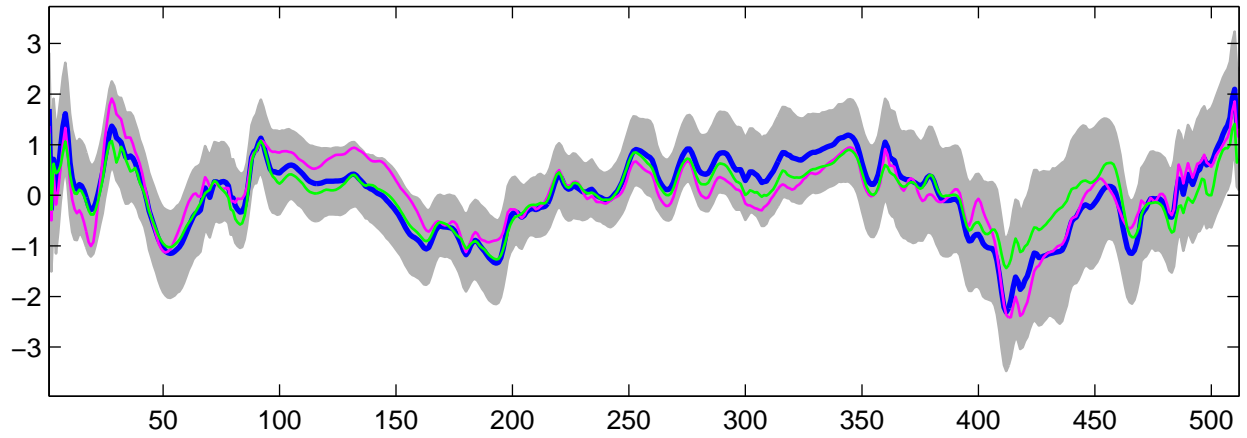
Estimated U_{22}(t) using G-WFMM: DE data, run 5
