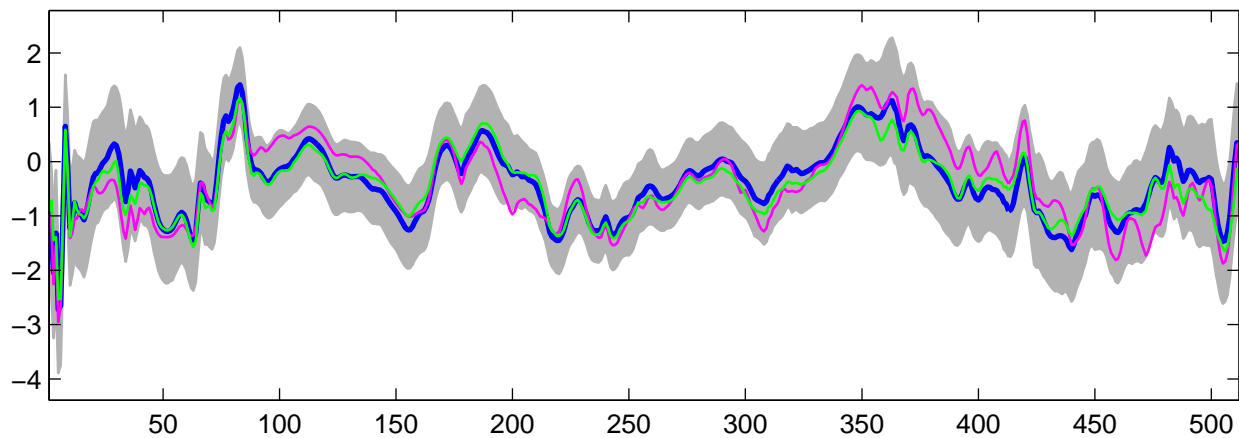
Estimated U_{22}(t) using G-WFMM: Normal data, run 5
