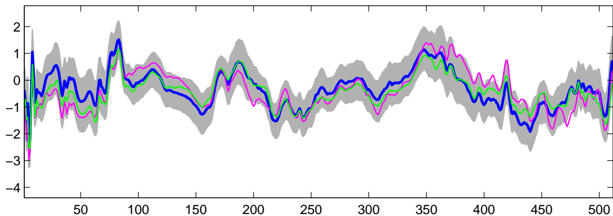
Estimated U_{22}(t) using R-WFMM: Normal data, run 5
