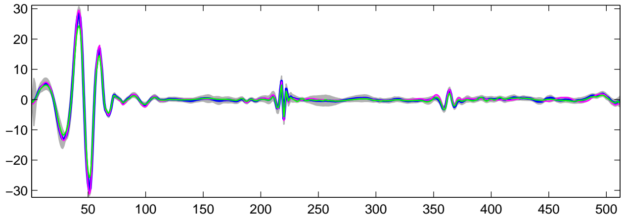
Estimated U_{22}(t) using G-WFMM: t_1 data, run 5
