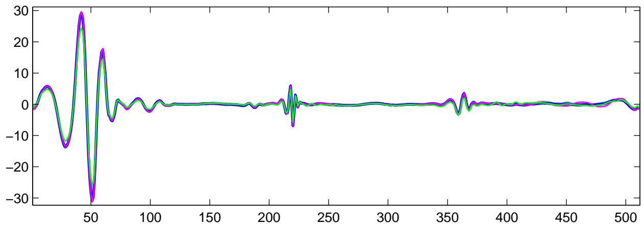
Estimated U_{22}(t) using R-WFMM: t_1 data, run 5
