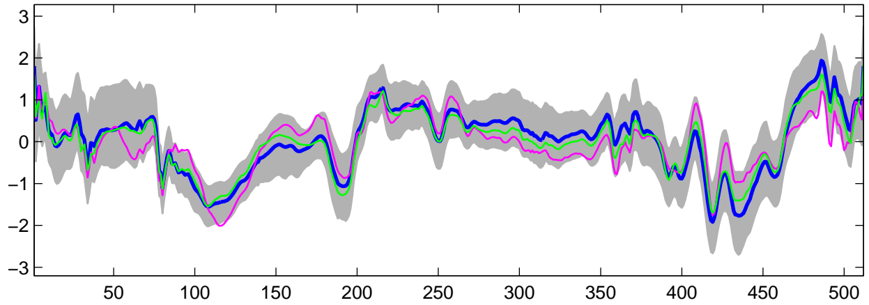
Estimated U_{22}(t) using G-WFMM: t_3 data, run 5
