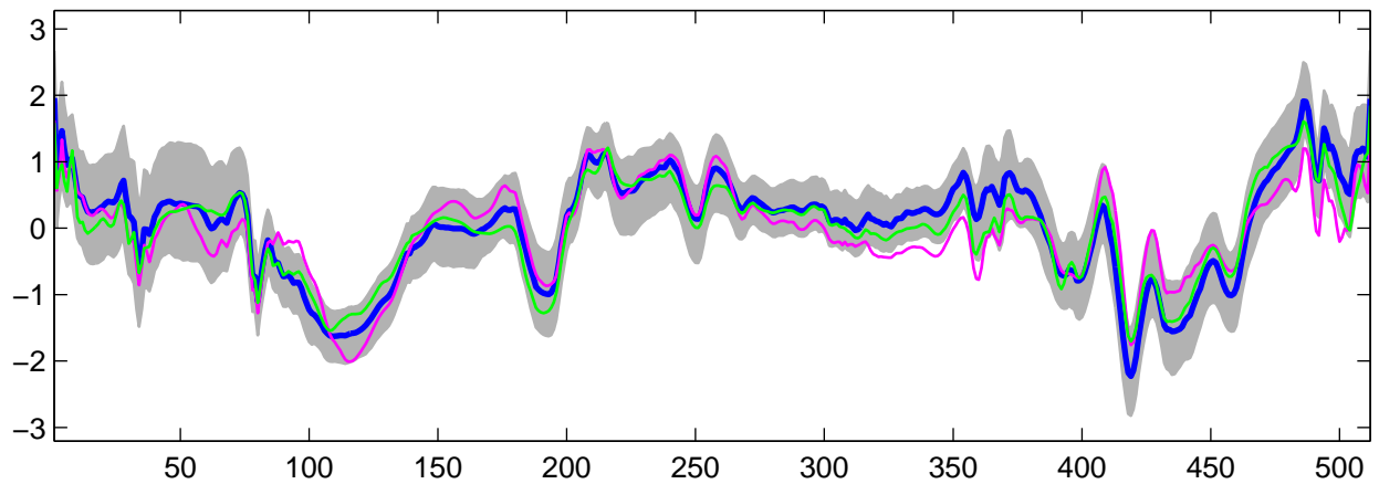
Estimated U_{22}(t) using R-WFMM: t_3 data, run 5
