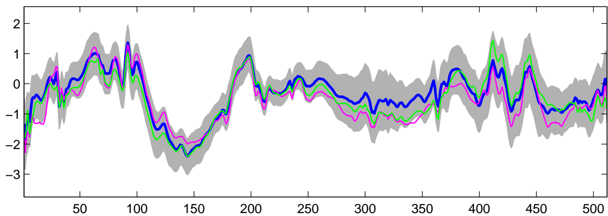
Estimated U_{23}(t) using R-WFMM: DE data, run 5
