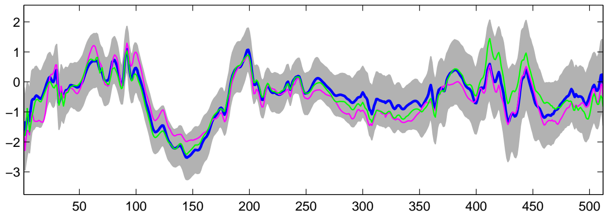
Estimated U_{23}(t) using G-WFMM: DE data, run 5
