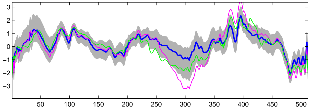
Estimated U_{23}(t) using R-WFMM: t_2 data, run 5
