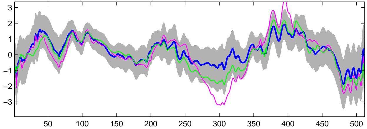
Estimated U_{23}(t) using G-WFMM: t_2 data, run 5
