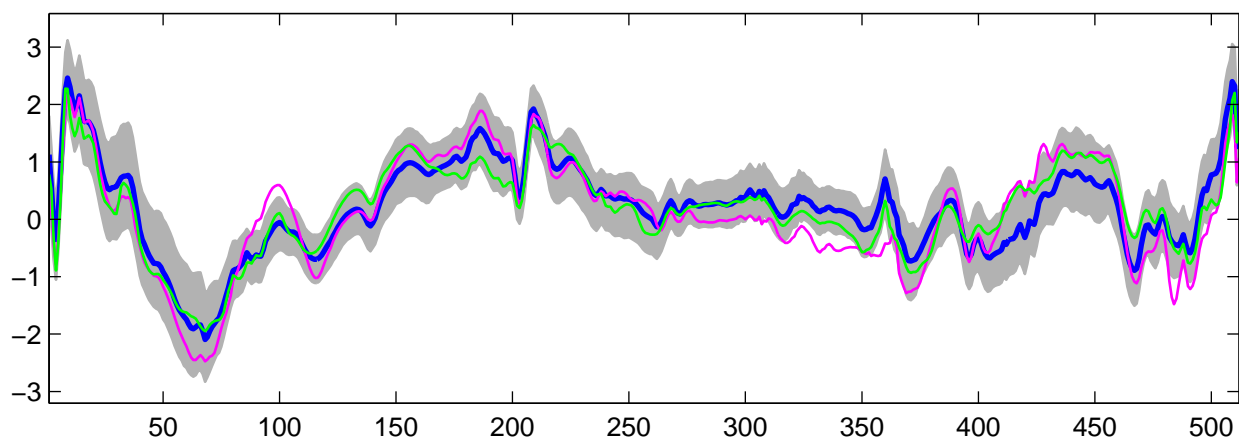
Estimated U_{23}(t) using R-WFMM: t_3 data, run 5
