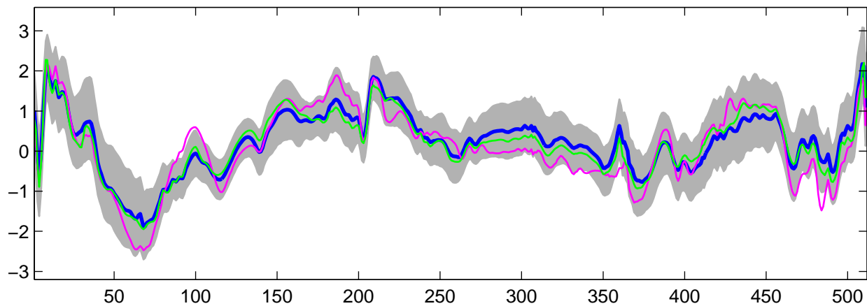
Estimated U_{23}(t) using G-WFMM: t_3 data, run 5
