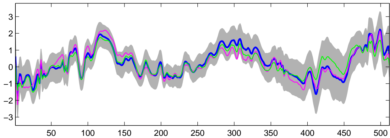
Estimated U_{24}(t) using G-WFMM: DE data, run 5
