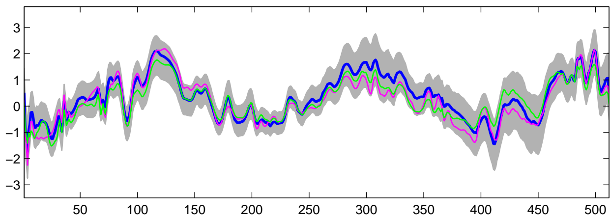
Estimated U_{24}(t) using R-WFMM: DE data, run 5
