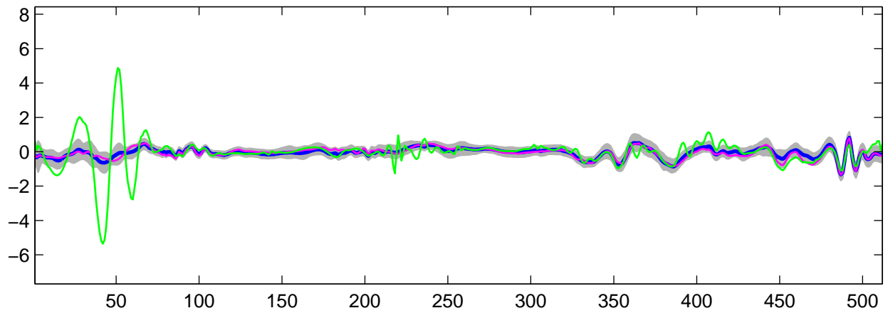
Estimated U_{24}(t) using R-WFMM: t_1 data, run 5
