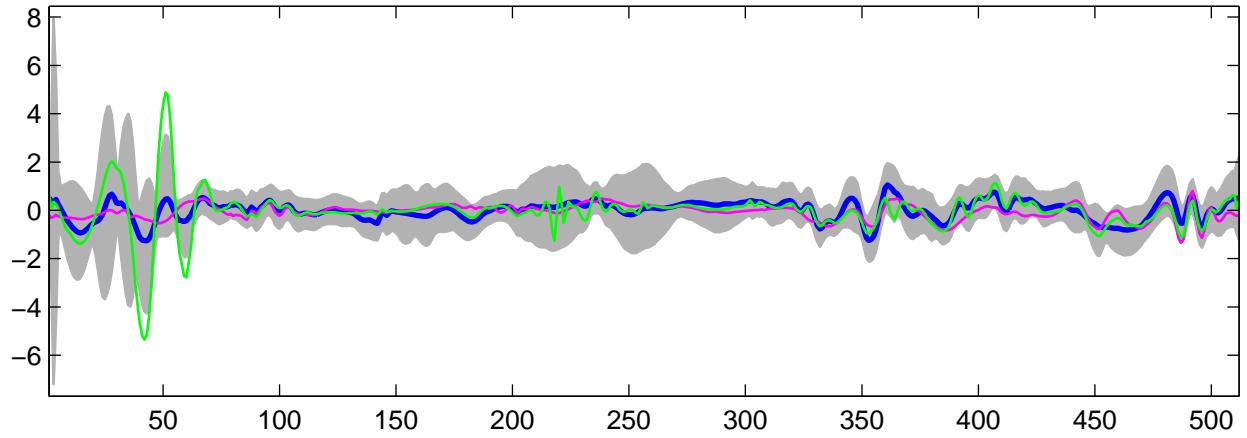
Estimated U_{24}(t) using G-WFMM: t_1 data, run 5
