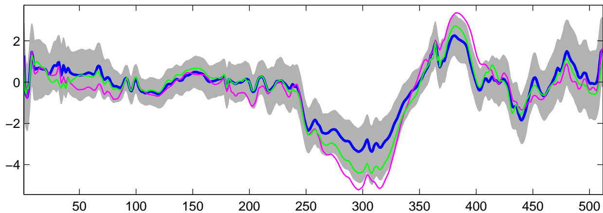
Estimated U_{24}(t) using G-WFMM: t_2 data, run 5
