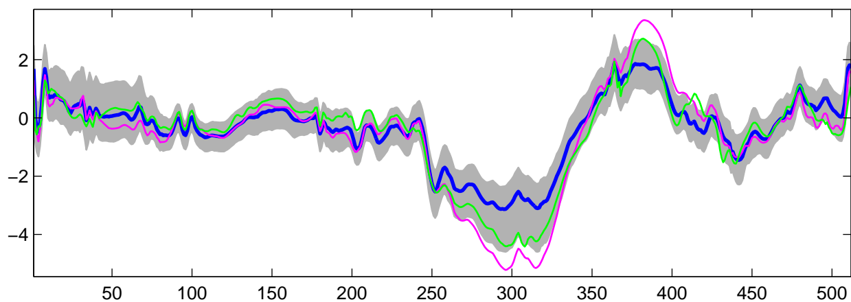
Estimated U_{24}(t) using R-WFMM: t_2 data, run 5
