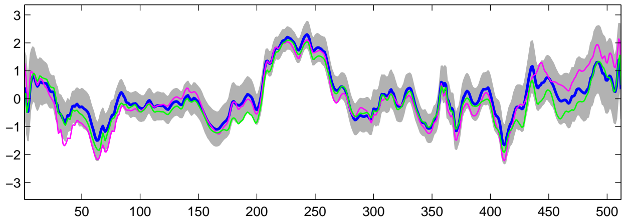
Estimated U_{25}(t) using R-WFMM: DE data, run 5
