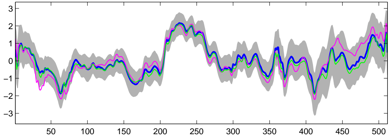
Estimated U_{25}(t) using G-WFMM: DE data, run 5
