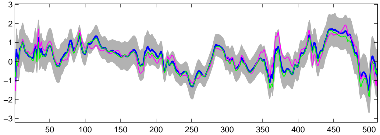
Estimated U_{25}(t) using G-WFMM: Normal data, run 5
