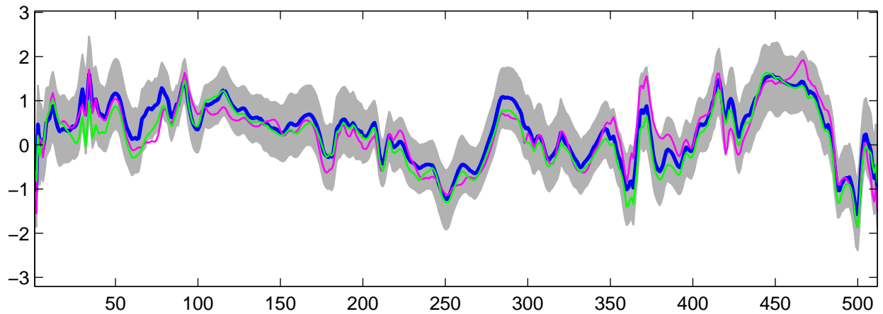
Estimated U_{25}(t) using R-WFMM: Normal data, run 5
