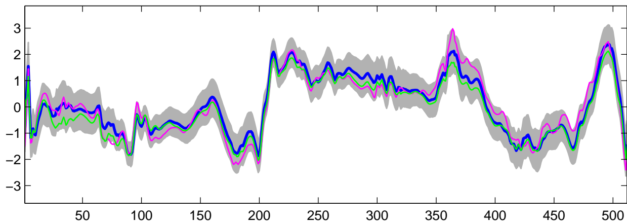
Estimated U_{26}(t) using R-WFMM: Normal data, run 5
