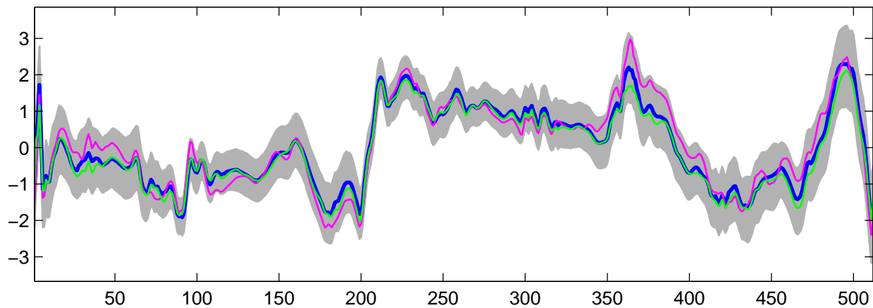
Estimated U_{26}(t) using G-WFMM: Normal data, run 5
