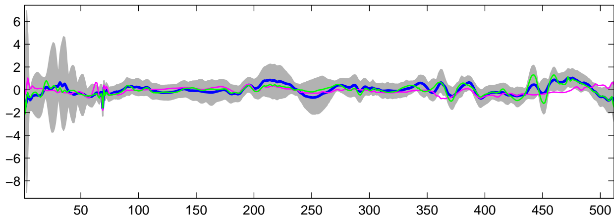
Estimated U_{26}(t) using G-WFMM: t_1 data, run 5
