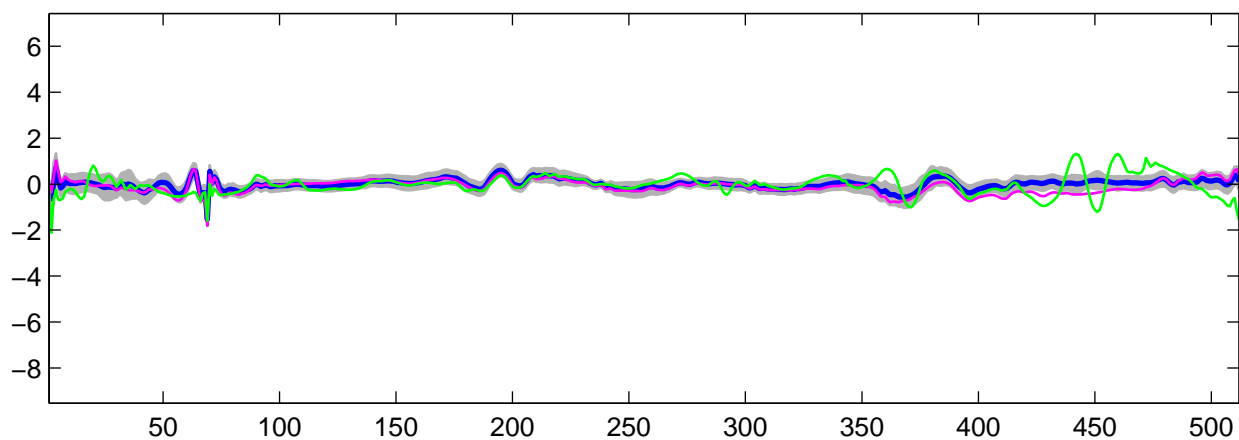
Estimated U_{26}(t) using R-WFMM: t_1 data, run 5
