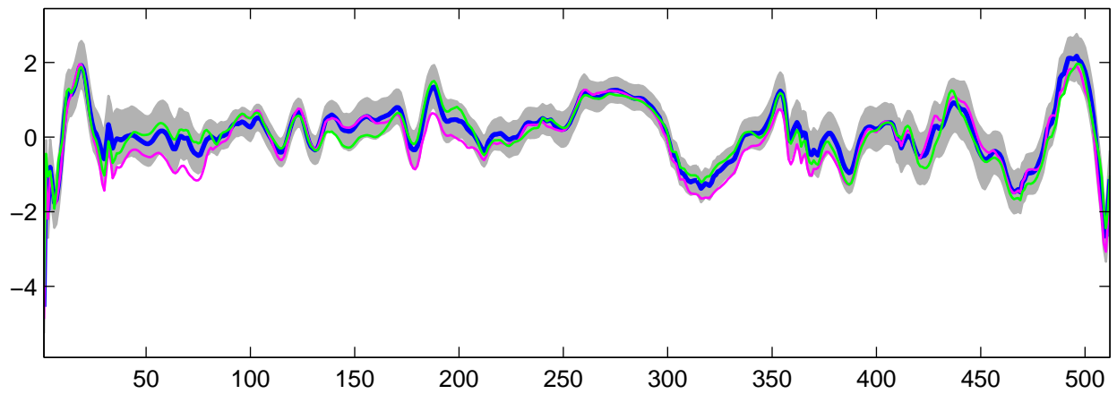
Estimated U_{26}(t) using R-WFMM: t_3 data, run 5
