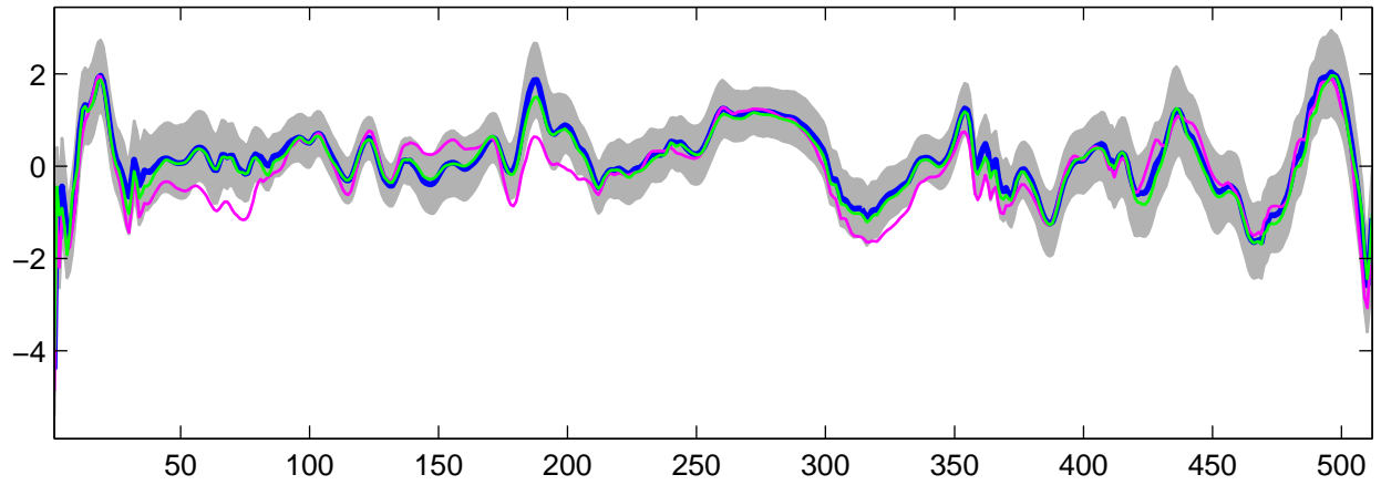
Estimated U_{26}(t) using G-WFMM: t_3 data, run 5
