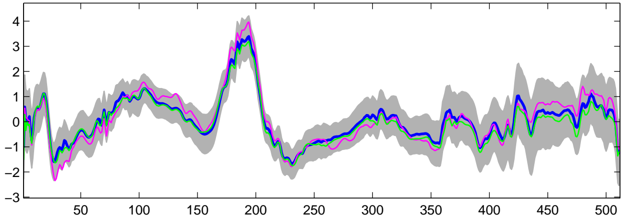
Estimated U_{27}(t) using G-WFMM: DE data, run 5
