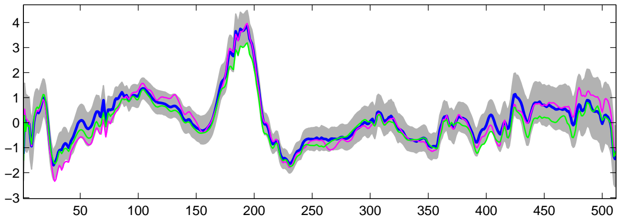
Estimated U_{27}(t) using R-WFMM: DE data, run 5
