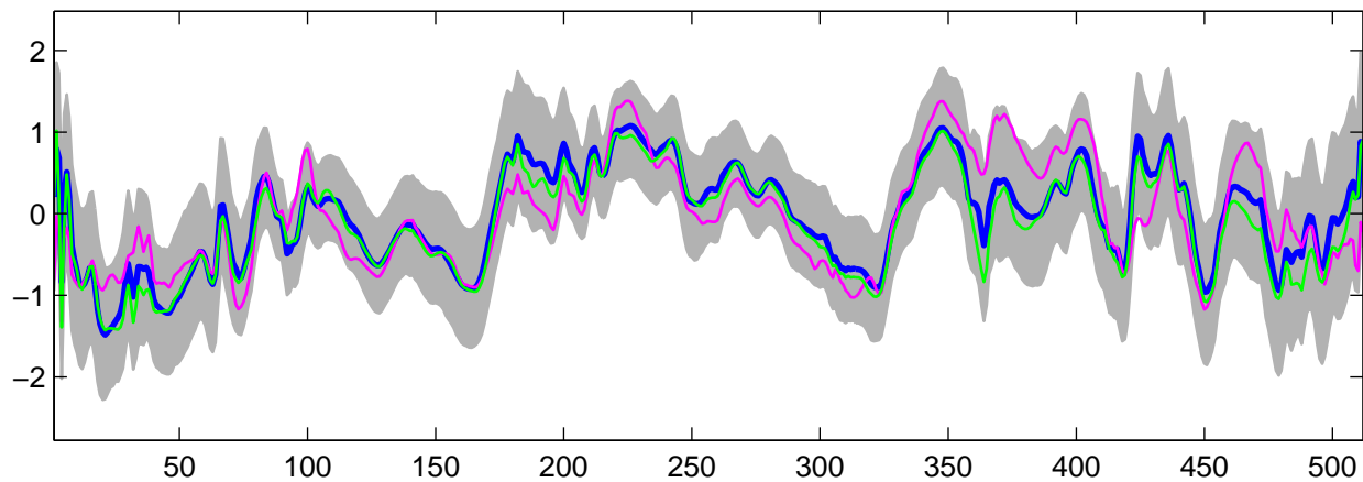
Estimated U_{27}(t) using G-WFMM: Normal data, run 5
