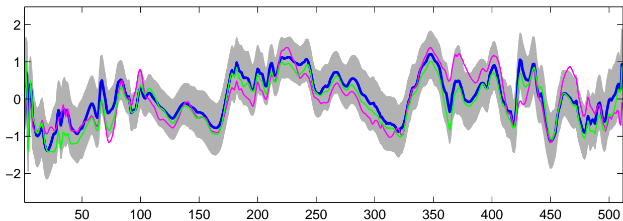
Estimated U_{27}(t) using R-WFMM: Normal data, run 5
