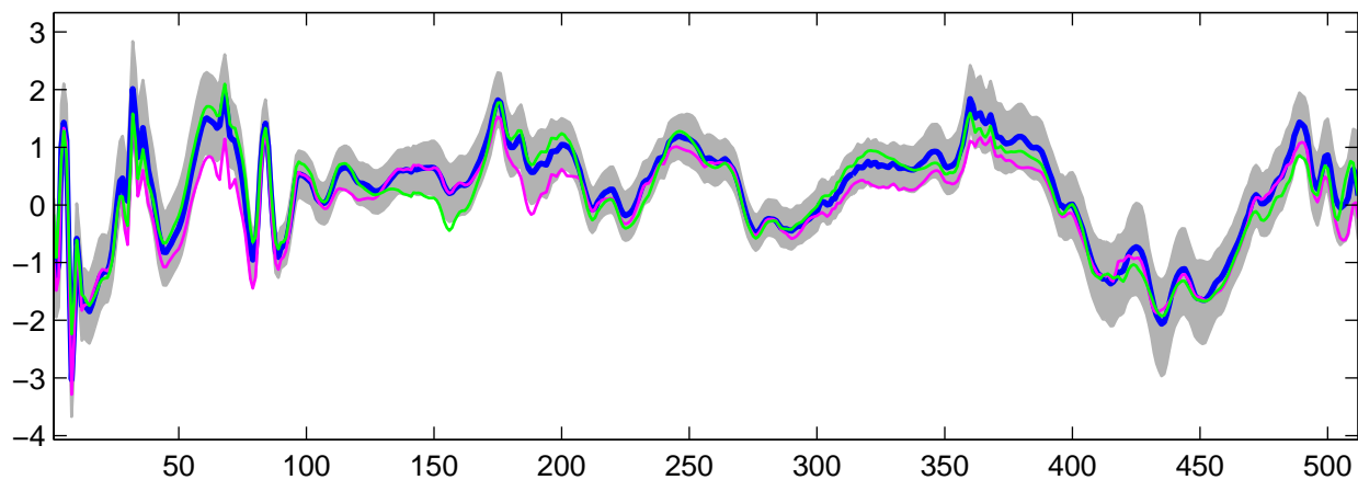
Estimated U_{27}(t) using R-WFMM: t_3 data, run 5
