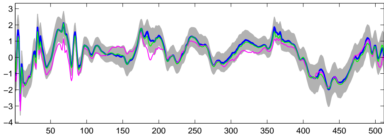
Estimated U_{27}(t) using G-WFMM: t_3 data, run 5
