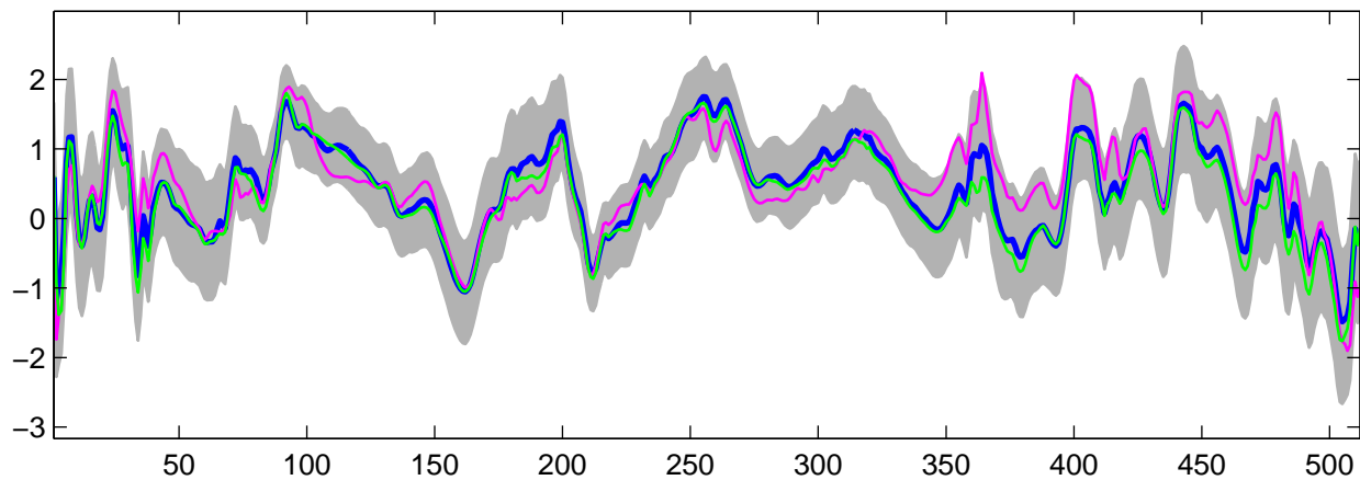
Estimated U_{28}(t) using G-WFMM: Normal data, run 5
