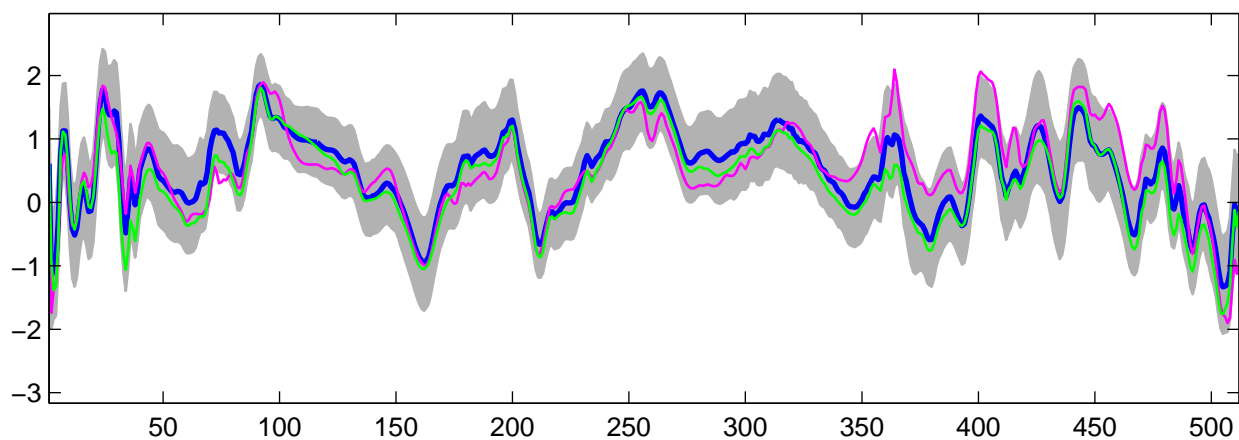
Estimated U_{28}(t) using R-WFMM: Normal data, run 5
