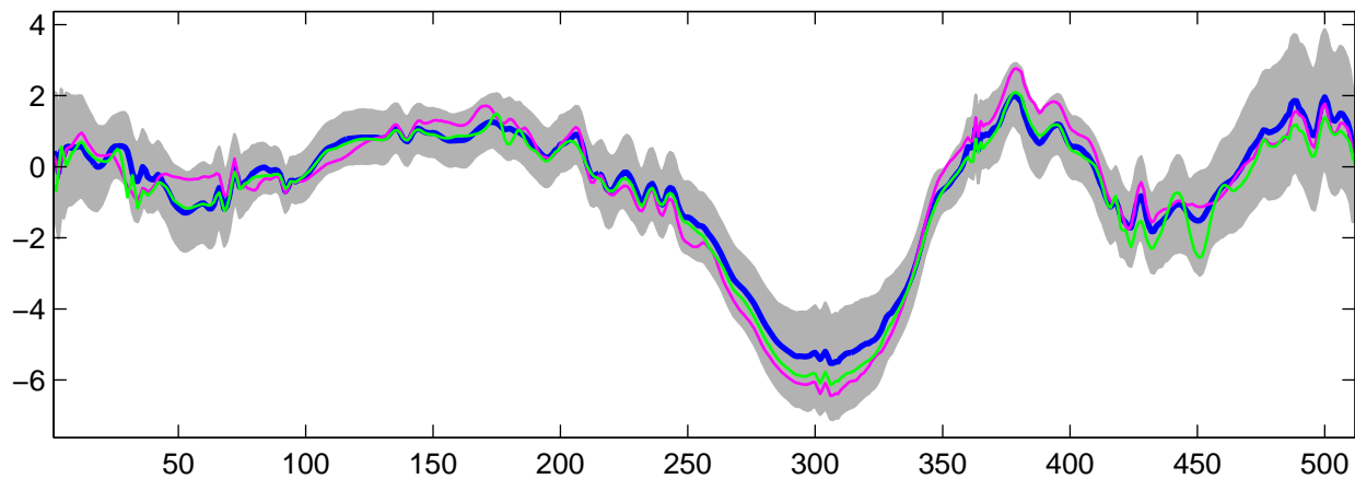
Estimated U_{28}(t) using G-WFMM: t_2 data, run 5
