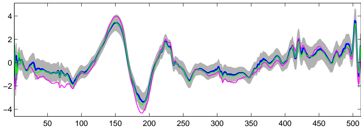
Estimated U_{28}(t) using G-WFMM: t_3 data, run 5
