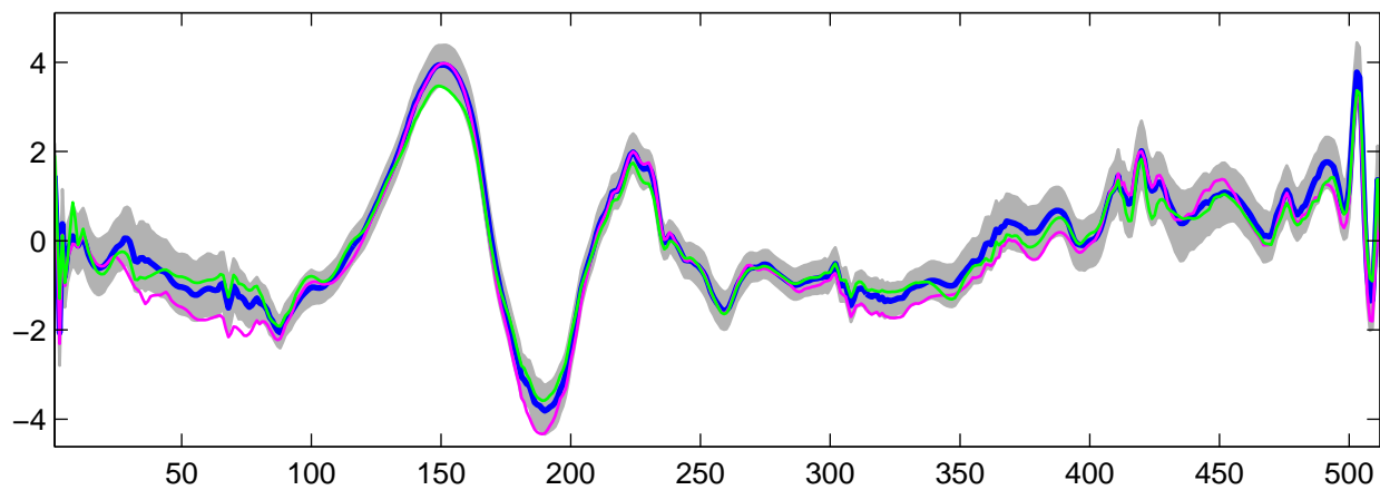
Estimated U_{28}(t) using R-WFMM: t_3 data, run 5
