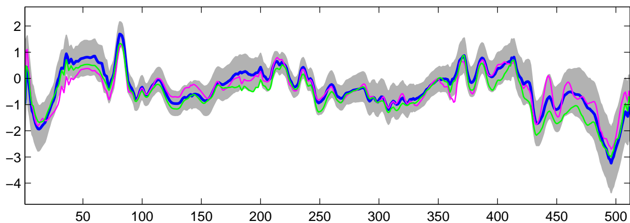
Estimated U_{29}(t) using R-WFMM: DE data, run 5
