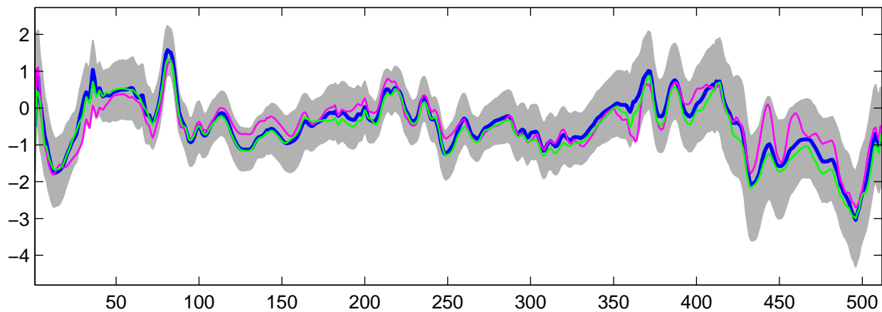
Estimated U_{29}(t) using G-WFMM: DE data, run 5
