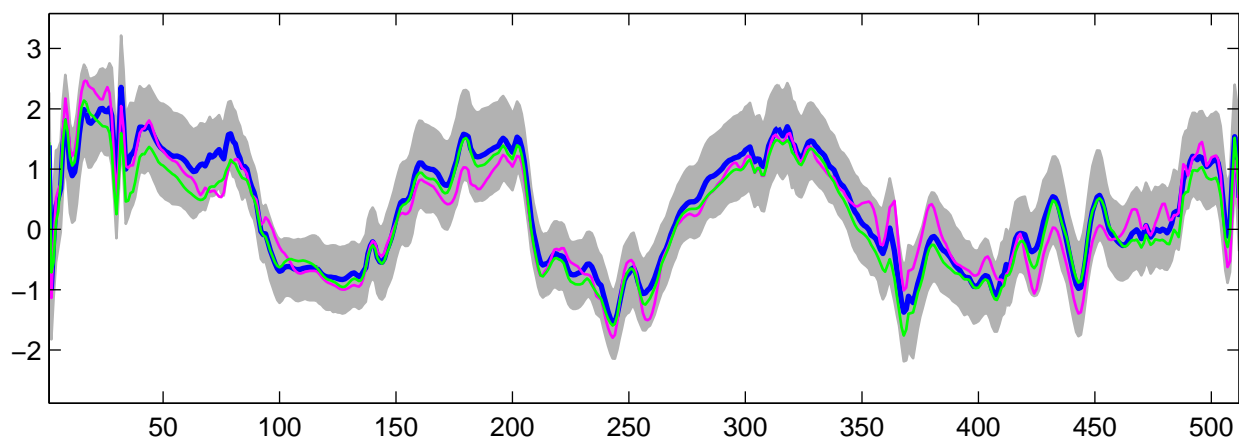
Estimated U_{29}(t) using R-WFMM: Normal data, run 5
