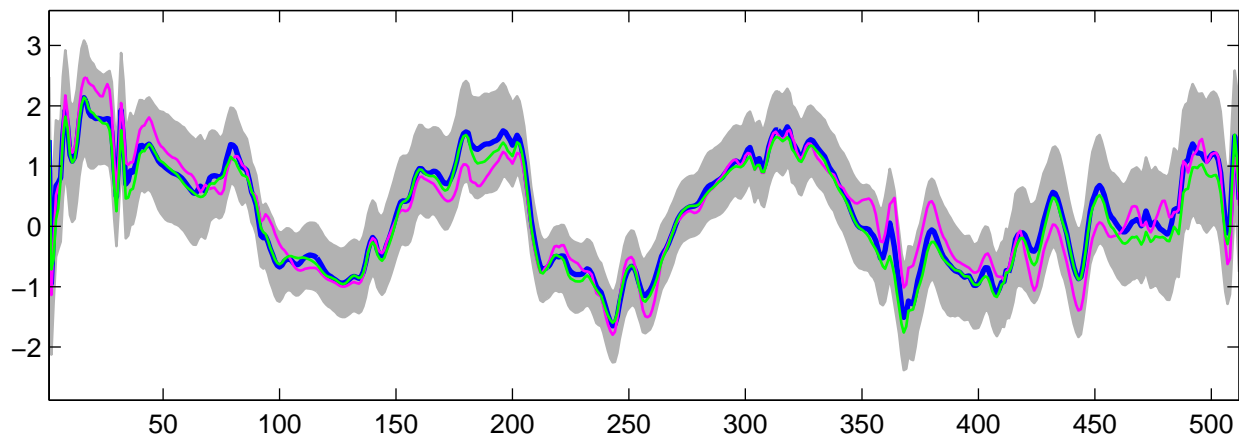
Estimated U_{29}(t) using G-WFMM: Normal data, run 5
