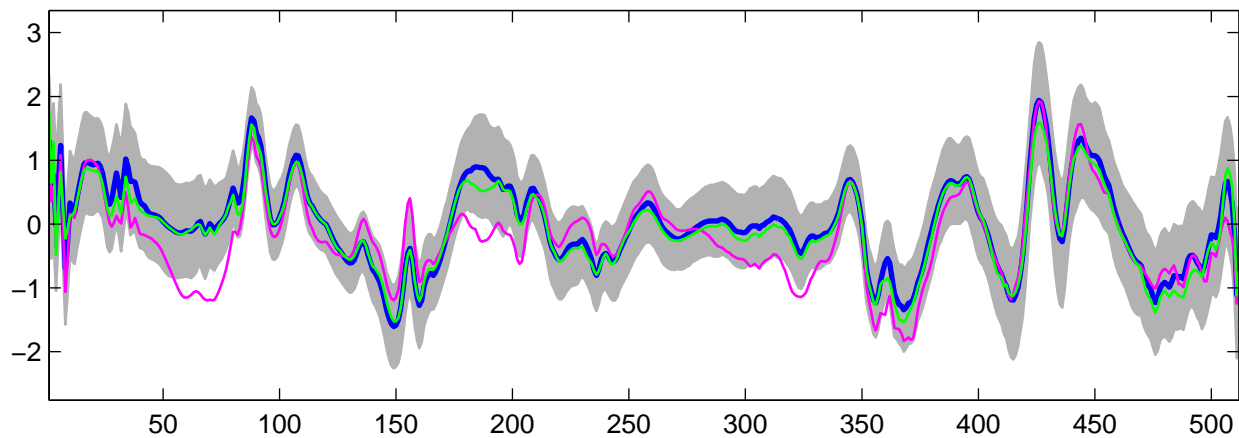
Estimated U_{29}(t) using G-WFMM: t_3 data, run 5
