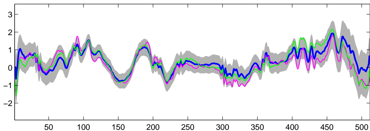
Estimated U_2(t) using R-WFMM: DE data, run 5
