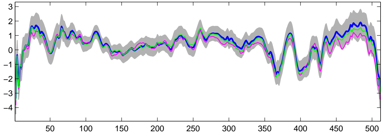
Estimated U_2(t) using G-WFMM: Normal data, run 5
