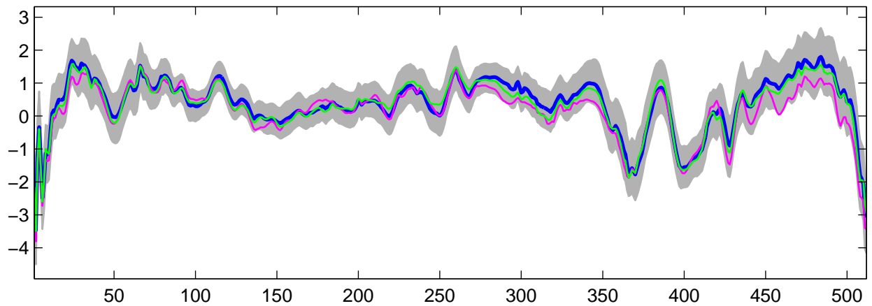
Estimated U_2(t) using R-WFMM: Normal data, run 5
