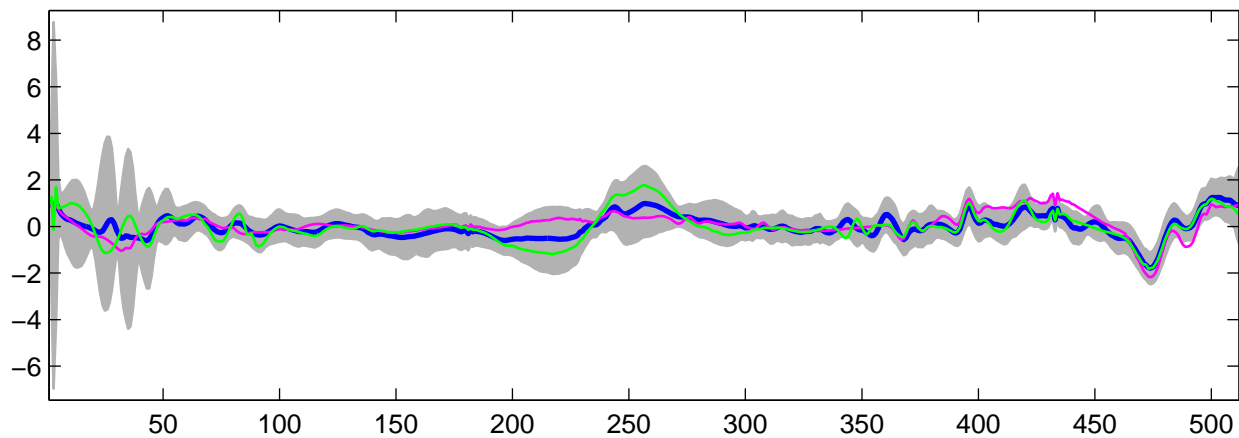
Estimated U_2(t) using G-WFMM: t_1 data, run 5
