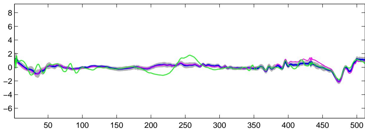
Estimated U_2(t) using R-WFMM: t_1 data, run 5
