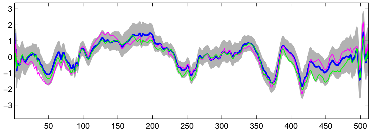
Estimated U_{30}(t) using R-WFMM: DE data, run 5
