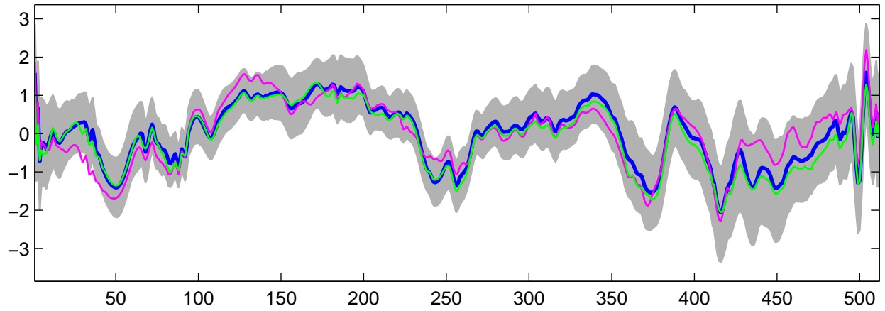
Estimated U_{30}(t) using G-WFMM: DE data, run 5
